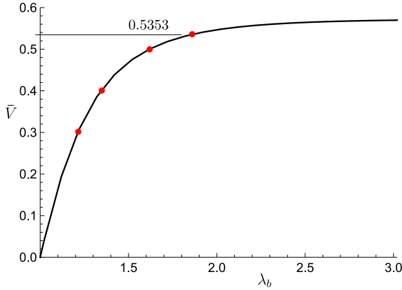
Fig. 12. Plot of \bar{V} versus \lambda_b for the parameters \alpha_\varepsilon = -0.3, \alpha_\mu = -0.3 and aspect ratio L/A = 10 . The red bullet points are associated with the values 0.3, 0.4, 0.5, 0.5353 of \bar{V} in Fig. 11(b)–(e), respectively.
