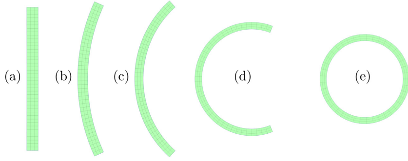
Fig. 11. (a) Undeformed rectangular plate cross section with aspect ratio L/A = 10 and parameters \alpha_\varepsilon = -0.3, \alpha_\mu = -0.3 and the following values of \bar{V} : (b) 0.3; (c) 0.4; (d) 0.5; (e) 0.5353.
