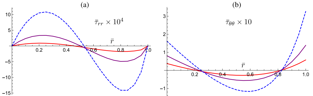
Fig. 8. Plots of (a) the radial stress \tau_{rr} and (b) the circumferential stress \tau_{\theta\theta} in scaled dimensionless form versus the normalized radius \bar{r} for the dimensionless voltage \bar{V} = 0.3 and the following values of (\alpha_\varepsilon, \alpha_\mu) : red (-0.3, 0.3) ; purple (-0.4, 0.3) ; blue dashed (-0.5, 0.3) . (For interpretation of the references to color in this figure legend, the reader is referred to the web version of this article.)
