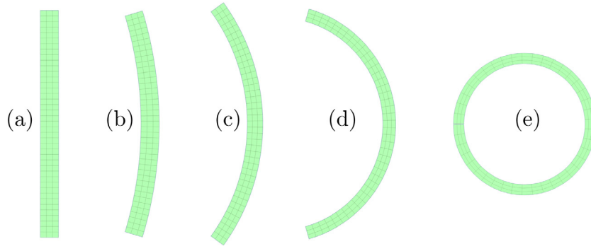
Fig. 2. (a) Undeformed rectangular plate cross section with aspect ratio L/A = 10 . (b)–(e) plate bent by application of a dimensionless voltage \bar{V} = 0.2 with the following values of (\alpha_\epsilon, \alpha_\mu) : (b) (0.3, 0.3); (c) (0.7, 0.3); (d) (1.1, 0.3); (e) (1.521, 0.3).
