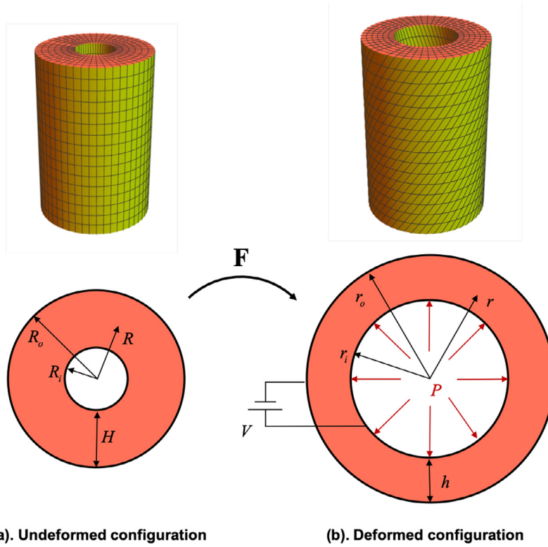
Fig. 2. Sketch of a DE tube in the (a) undeformed and (b) deformed configurations. The upper row presents three dimensional images of the tubes and the lower row shows the associated in-plane cross sections.
