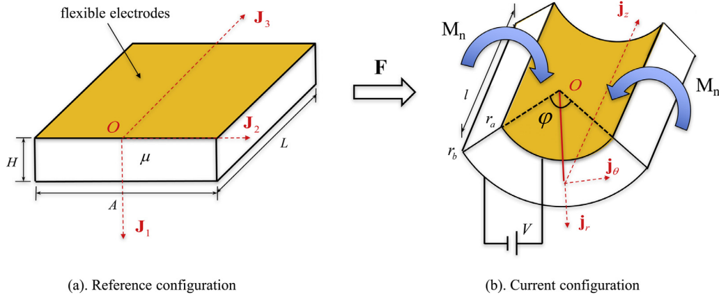
Fig. 2. Sketch of a dielectric slab with a voltage applied across its thickness subject to finite bending.
