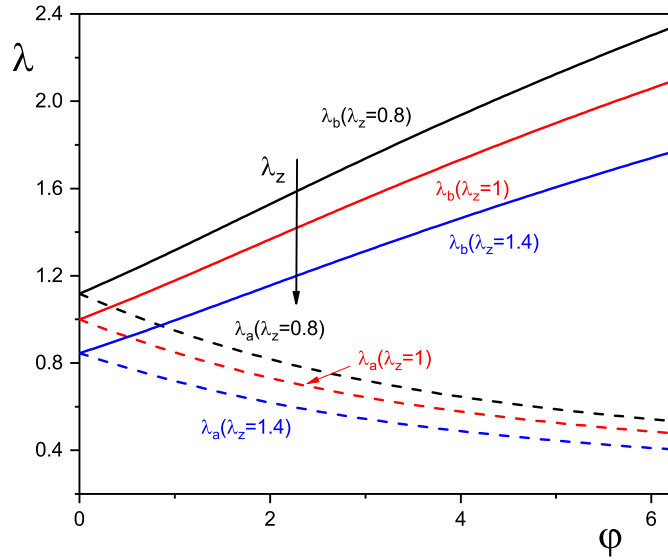
Fig. 6. Plots of \lambda_a, \lambda_b - \varphi for fixed axial compressions \lambda_z = 0.8, 1, 1.4 of dielectric slabs with \bar{V} = 0, A/H = 3 .
