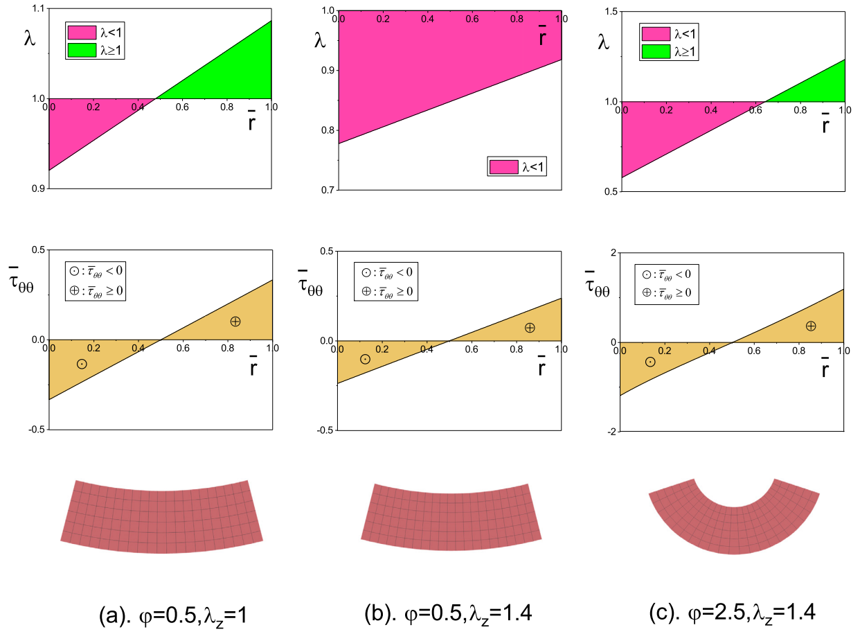
Fig. 8. Purely elastic bending of a dielectric slab which is three times wider than thick ( \bar{V} = 0, A/H = 3 ) for various bending angles and axial elongation ratios: (a) \bar{\varphi} = 0.5, \lambda_z = 1 ; (b) \bar{\varphi} = 0.5, \lambda_z = 1.4 ; (c) \bar{\varphi} = 2.5, \lambda_z = 1.4 . The top, middle and bottom rows show the variations through the thickness of the circumferential stretch and of the stress distributions, and the resulting bending shapes, respectively.
