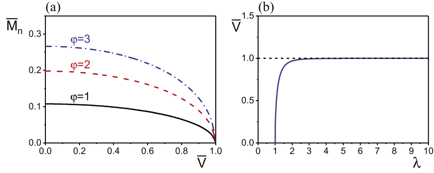
Fig. 5. (a) Plots of \bar{M}_n - \bar{V} for several specific bending angles \varphi = 1, 2, 3 of a dielectric slab which is three times wider than thick, and no axial compression ( \lambda_z = 1, A/H = 3 ); (b) Nonlinear response of a dielectric slab subject to a voltage.
