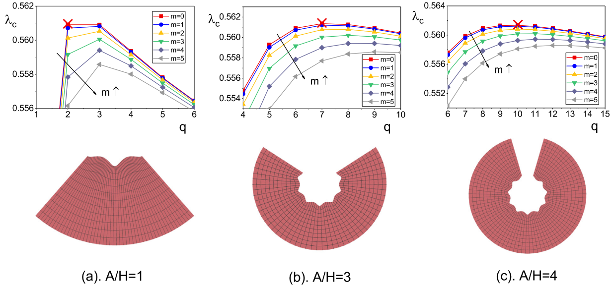
Fig. 10. Elastic bending instability of a dielectric slab with fixed axial compression ( \bar{V} = 0 , \lambda_z = 1 ) for various width aspect ratios: (a) A/H = 1 ; (b) A/H = 3 ; (c) A/H = 4 and fixed length aspect ratio L/H = 10 . The top row shows plots of the critical circumferential stretch \lambda_c versus the number of circumferential wrinkles q for a range of axial modes m = 0 - 5 . The bottom row shows the corresponding wrinkling shapes when instability occurs. The highest point of \lambda_c - q curves for each case is marked by cross, representing the onset of the instability. In this case the m = 0 plot is always on top and there are no axial wrinkles, only circumferential.
