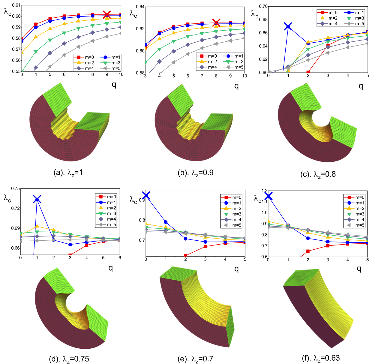
Fig. 14. Bending instability of dielectric slabs with A/H = 3 , L/H = 1.5 , \bar{V} = 0.3 and subject to (a) \lambda_z = 1 ; (b) \lambda_z = 0.9 ; (c) \lambda_z = 0.8 ; (d) \lambda_z = 0.75 ; (e) \lambda_z = 0.7 ; (f) \lambda_z = 0.63 . The top rows are plots of \lambda_c versus q for a range of modes m = 0 - 5 and bottom rows are the corresponding wrinkling shapes when instability occurs. In cases (a) and (b), circumferential wrinkles occurs and in cases (e) and (f), axial wrinkles occurs whereas in cases (c) and (d), a two dimensional (circumferential and axial) pattern emerges.
