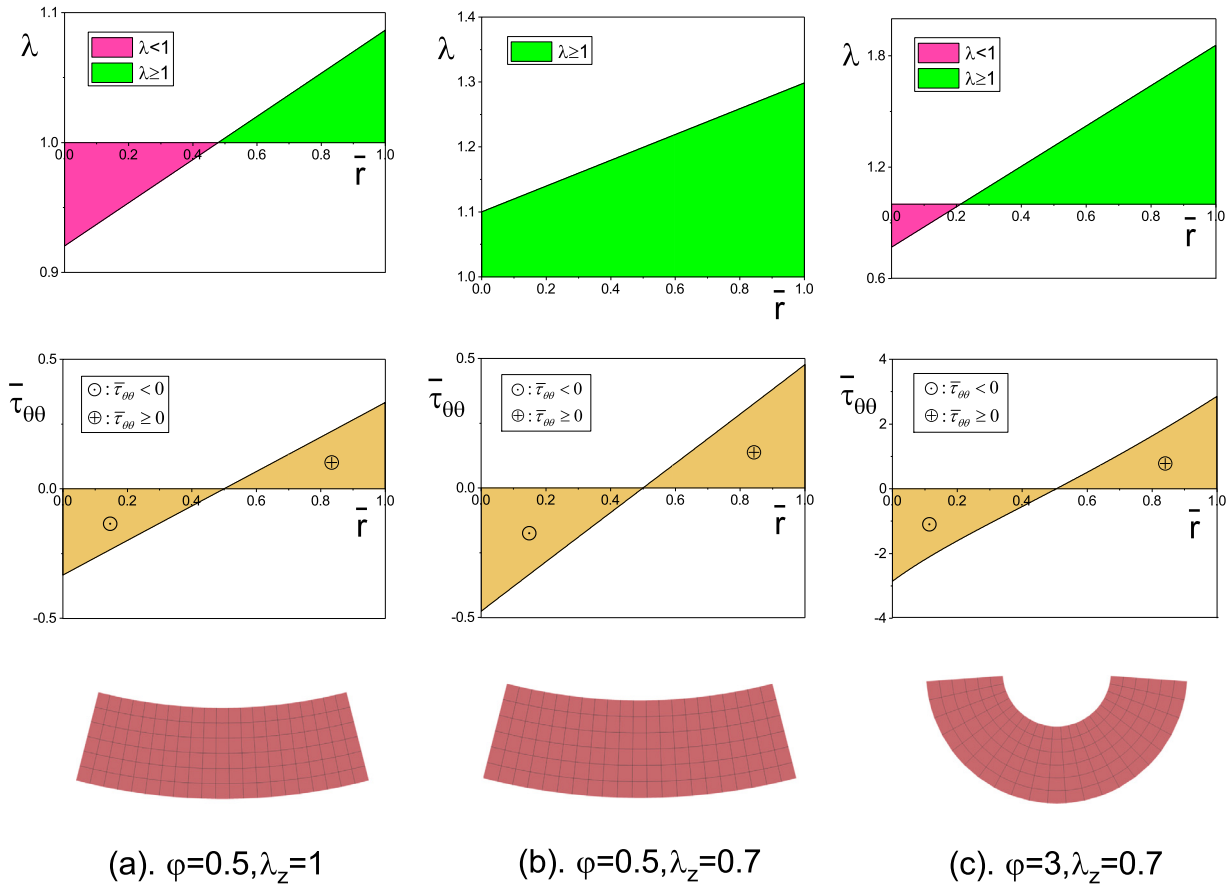
Fig. 7. Purely elastic bending of a dielectric slab which is three times wider than thick ( \bar{V}=0, A/H=3 ) for various bending angles and axial compression ratios: (a) \varphi=0.5, \lambda_z=1 ; (b) \varphi=0.5, \lambda_z=0.7 ; (c) \varphi=3, \lambda_z=0.7 . The top, middle and bottom rows show the variations through the thickness of the circumferential stretch and of the stress distributions, and the resulting bending shapes, respectively.
