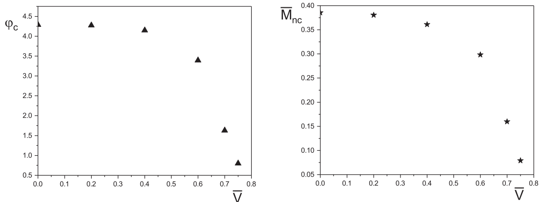
Fig. 13. Effect of the applied voltage \bar{V} on the critical values of bending angle \phi_c and moment \bar{M}_{nc} for dielectric slabs with A/H = 3, L/H = 1.5, \lambda_z = 0.85 .
