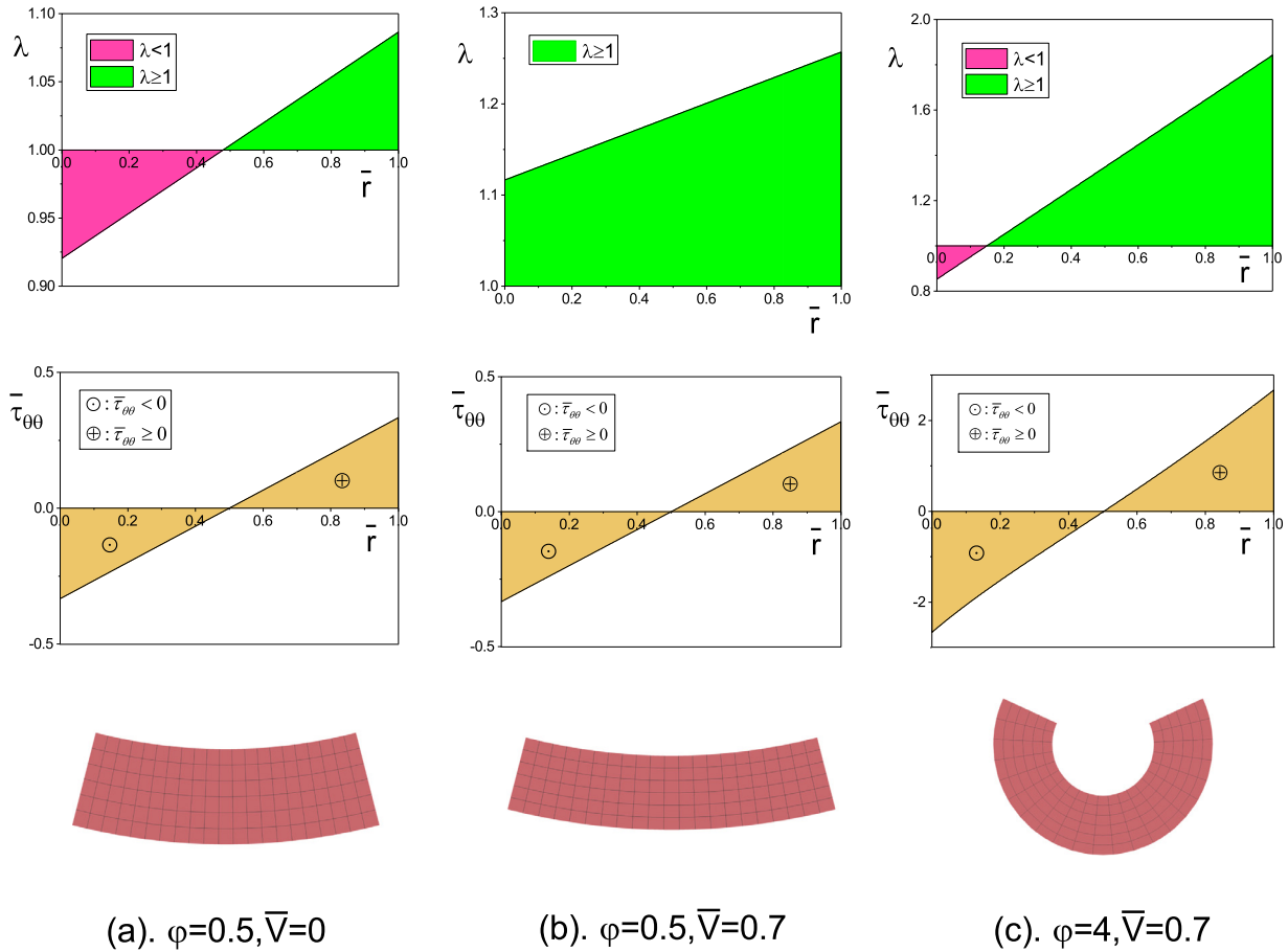
Fig. 4. Bending of dielectric slabs which are three times wider than thick, with no axial compression ( \lambda_z = 1, A/H = 3 ) and subject to various bending angles and voltage loadings: (a) \phi = 0.5, \bar{V} = 0 ; (b) \phi = 0.5, \bar{V} = 0.7 ; (c) \phi = 4, \bar{V} = 0.7 . The top, middle and bottom rows correspond to the circumferential stretch, circumferential stress distributions, and bending shapes, respectively.
