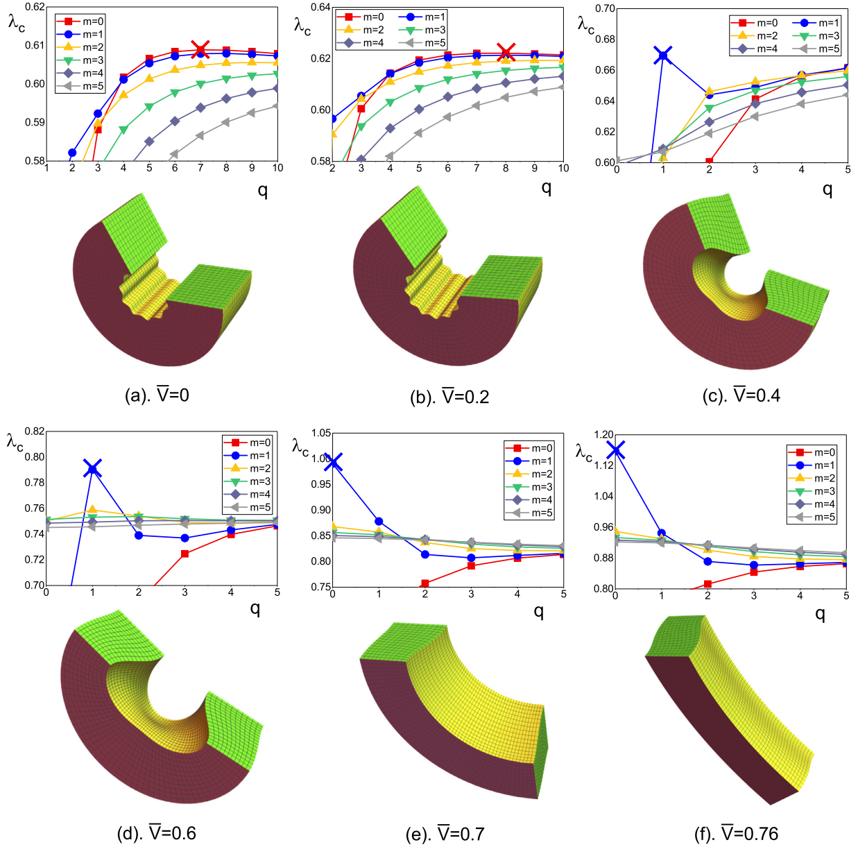
Fig. 12. Bending instability of compressed dielectric slabs which are 3 times wider and 1.5 times taller than thick ( A/H = 3, L/H = 1.5, \lambda_z = 0.85 ) and subject to increasing voltages: (a) \bar{V} = 0 ; (b) \bar{V} = 0.2 ; (c) \bar{V} = 0.4 ; (d) \bar{V} = 0.6 ; (e) \bar{V} = 0.7 ; (f) \bar{V} = 0.76 . The top rows are plots of \lambda_c versus q for a range of modes m = 0 - 5 and bottom rows are the corresponding wrinkling shapes when instability occurs. In cases (a) and (b), circumferential wrinkles occurs and in cases (e) and (f), axial wrinkles occurs whereas in cases (c) and (d), a two-dimensional (circumferential and axial) pattern emerges.
