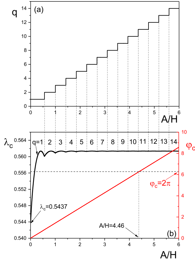
Fig. 11. (a) Critical circumferential mode number q and (b) stretch \lambda_c (evaluated at the inner face of the bent sector r_a ) and critical bending angle \varphi_c versus width aspect ratio A/H of an elastic slab ( \bar{V} = 0 ) under bending only ( \lambda_z = 1 ) at the onset of buckling.
