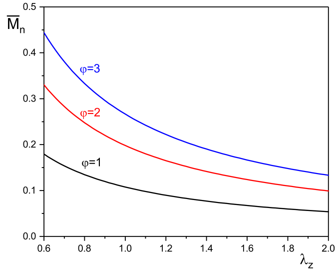
Fig. 9. Plots of \bar{M}_n - \lambda_z for bending angle \varphi = 1, 2, 3 of a dielectric slab with \bar{V} = 0, A/H = 3 .
