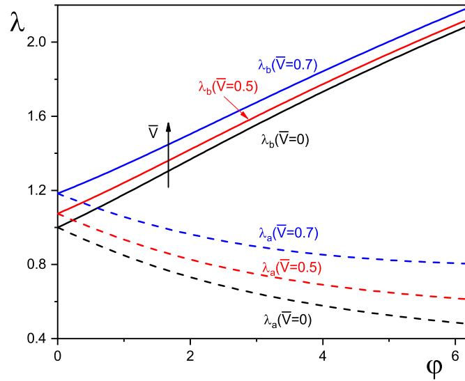
Fig. 3. Plots of \lambda_a, \lambda_b - \phi for dielectric slabs with \lambda_z = 1, A/H = 3 subject to voltage \bar{V} = 0, 0.5, 0.7 , respectively.
