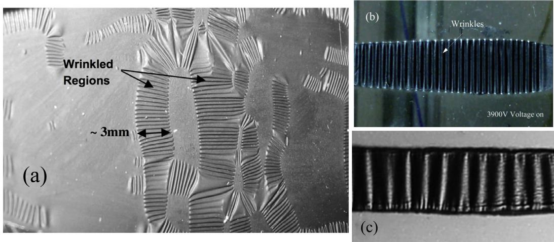
Fig. 2. Experimental evidence of electro-mechanical wrinkling instability: (a) collapse of a thin film of the rubber-like material VHB 4905/4910 put under a large voltage (Plante and Dubowsky, 2006); (b) wrinkling of a VHB 4910 membrane under high voltage (Liu et al., 2016); (c) electric activation of acrylic elastomers (Pelrine et al., 2000). We estimate that the ratio of the initial plate thickness to the wrinkle wavelength is H/\mathcal{L} \simeq 0.17, 0.35 in Cases (a) and (b), respectively.
