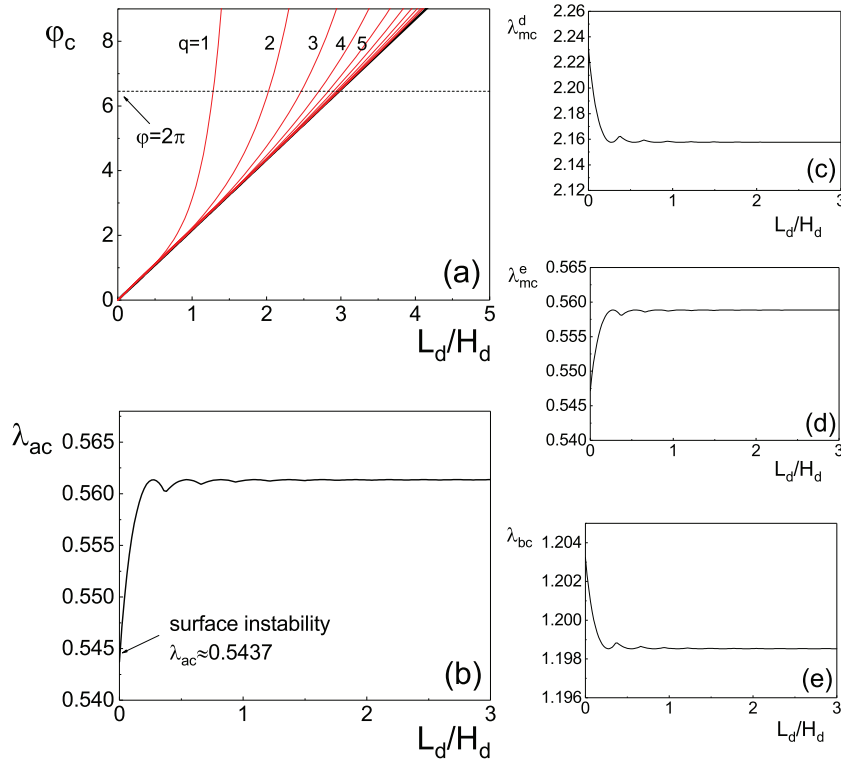
Fig. 7. Bending instability of a neo-Hookean ( G^d = G^e = 10^4 ) dielectric-elastomeric bilayer with \bar{H} = \bar{\mu} = 1 : the critical bending angle \phi_c and the critical stretches \lambda_{ac} , \lambda_{mc}^d , \lambda_{mc}^e and \lambda_{bc} at the onset of buckling versus the width aspect ratio of the dielectric elastomer L^d/H^d are shown in (a)–(e), respectively.
