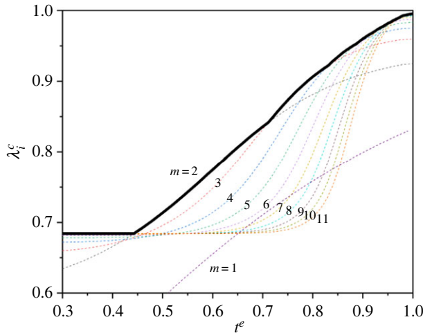
Figure 4. Plots of the critical strains of a Gent elastic balloon as functions of the radius ratio t^e , shown at different buckling modes m = 1, 2, \dots, 11 (dashed lines). The bold black line corresponds to the marginal stability curve.
