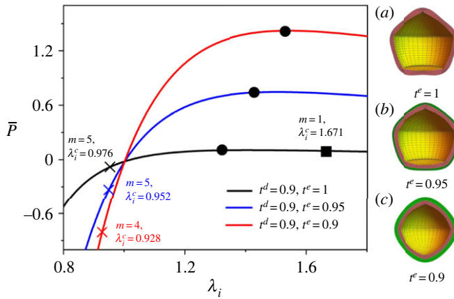
Figure 8. Inflation and buckling responses of pressure activated ( \bar{V} = 0.3 ) dielectric-elastic balloons with t^d = 0.9 and varying t^e . The \bar{P} - \lambda_i curve is shown on the left, and the buckling shapes are shown on the right (a–c). The cross, circle and square markers indicate the thresholds for buckling in compression, snap-through and buckling in extension, respectively.
