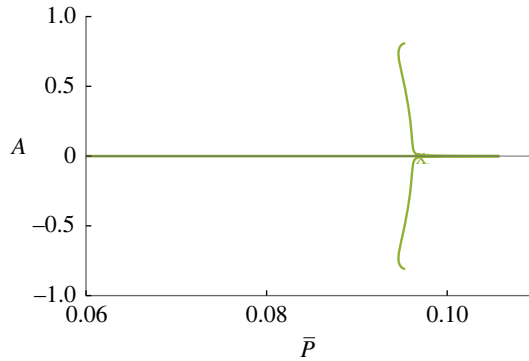
Figure 12. Bifurcation diagram showing \bar{P} versus the dimensionless amplitude of the deformation on the free surface A for \bar{V} = 0.3 , \mu^e/\mu^d = 10 , t^d = 0.9 , and t^e = 1 , \bar{V} = 0.3 . The marker cross denotes the theoretical buckling threshold.
