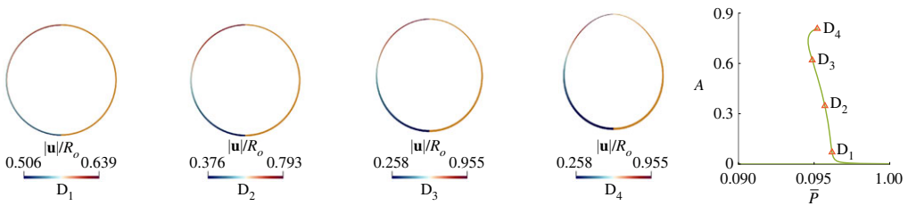
Figure 13. (left) Plot of the actual configuration of DE balloons, with t^d = 0.9 , \mu^e/\mu^d = 10 , \bar{V} = 0.3 . Here, we show a planar section of the balloon, where on the left we show ||u||/R_o , while on the right each layer is identified using different colours (orange: DE, blue: elastomer). On the right, we show the corresponding points to each configuration on the bifurcation diagram.
