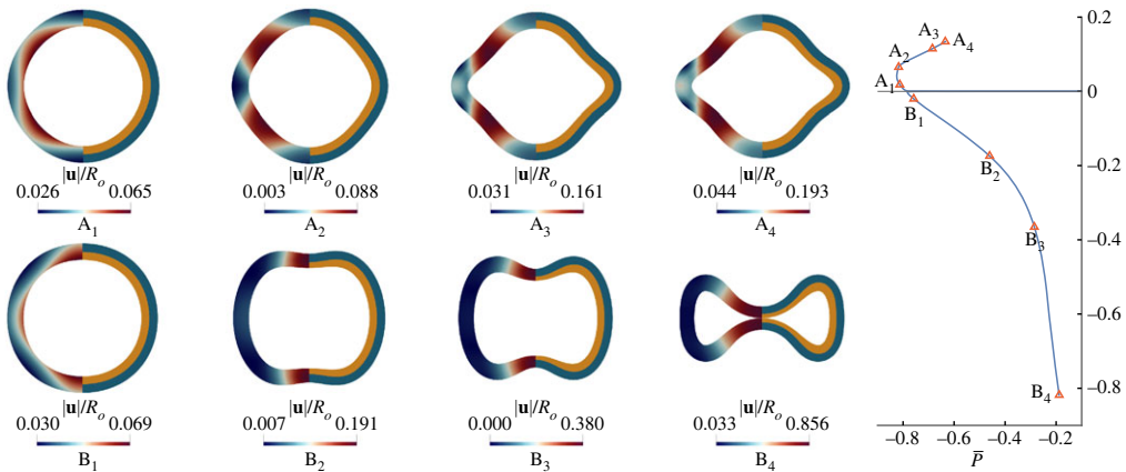
Figure 10. (left) Plot of the actual configuration of the planar section of spherical bilayers, with t^d = 0.9 , t^e = 0.9 , \mu^e/\mu^d = 10 . Here, we show a section of the shell, where on the left we show \|u\|/R_o , while on the right each layer is identified using different colours (orange: DE, blue: elastomer). On the right, we show the corresponding points to each configuration on the bifurcation diagram.
