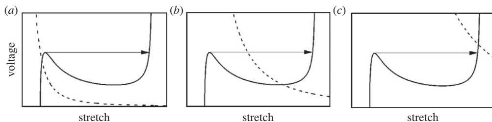
Figure 1. Nonlinear responses of planar DE actuators subject to a voltage through the thickness: (a) electrical breakdown occurs prior to the onset of snap-through instability (type I); (b) snap-through instability induces electrical breakdown of the material (type II); and (c) the DEs survive the snap-through instability (type III). The solid and dashed curves correspond to the voltage-stretch loading curve and the electric breakdown curve of the materials, respectively. The arrow represents the snap-through path of the material during the deformation.
