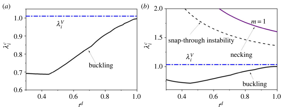
Figure 6. Plots of the critical strains versus the radius ratio t^d for a single layer of DE ( t^e = 1 ): (a) \bar{V} = 0.1 and (b) \bar{V} = 0.3 . The black dashed line depicts the snap-through instability threshold, the blue dot-dashed line depicts the inner circumferential stretch \lambda_i^V of the balloon induced by the applied voltage only, i.e. considering \bar{P} = 0 . The magenta solid line finally depicts the threshold for necking. For simplification, here we do not show the instability thresholds for the different modes m = 1, 2, \dots, 11 (dashed lines as in figure 4), but only present the actual marginal stability curve.
