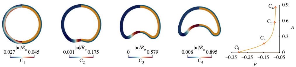
Figure 11. (left) Plot of the actual configuration of the planar section of spherical bilayers, with t^d = 0.9 , t^e = 0.95 , \mu^e/\mu^d = 10 , \bar{V} = 0.3 . Here, we show a section of the shell, where on the left we show \|u\|/R_o , while on the right each layer is identified using different colours (orange: DE, blue: elastomer). On the right, we show the corresponding points to each configuration on the bifurcation diagram.
