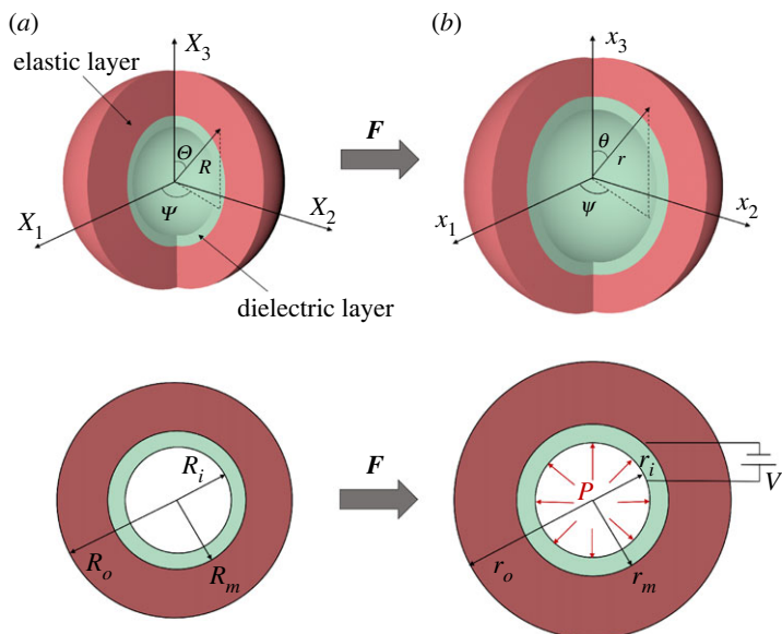
Figure 2. Sketch of a layered dielectric-elastic balloon subject to a radial voltage V through the DE layer and an internal pressure P at the inner surface: (a) undeformed and (b) deformed configurations. The upper row depicts the three-dimensional domains with the respective spherical coordinate systems, and the lower row shows the corresponding in-plane cross sections with geometrical and electro-mechanical loading parameters.
