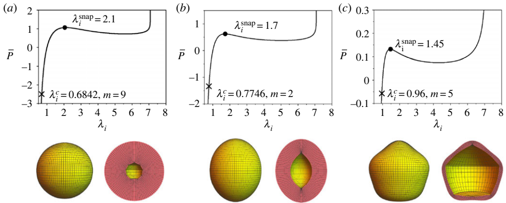
Figure 3. Inflation and buckling responses of (a) thick, (b) moderately thick and (c) thin elastic balloons ( \bar{V} = 0 , t^d = 1 ), respectively. The cross and circle markers indicate the thresholds for buckling in compression and snap-through instabilities of the material, respectively. The upper row presents the \bar{P} - \lambda_i curve, and the lower row shows the shape of the balloon at the onset of buckling. Note that we have set a finite amplitude of the incremental displacement for the sake of graphical illustration of the buckling pattern. (a) t^e = 0.4 , (b) t^e = 0.6 and (c) t^e = 0.9 .
