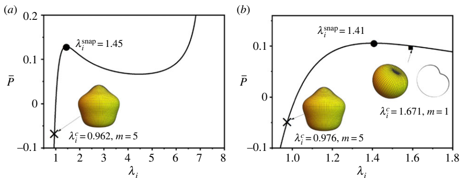
Figure 5. Inflation and buckling responses of thin DE balloons ( t^e = 1 , t^d = 0.9 ) subject to a fixed voltage: (a) \bar{V} = 0.1 and (b) \bar{V} = 0.3 . The cross, circle and square markers indicate the thresholds for buckling in compression, snap-through and buckling in extension instabilities of the material, respectively. Inset: the shape of the balloon at the onset of buckling; and the sectional view of the balloon at necking.
