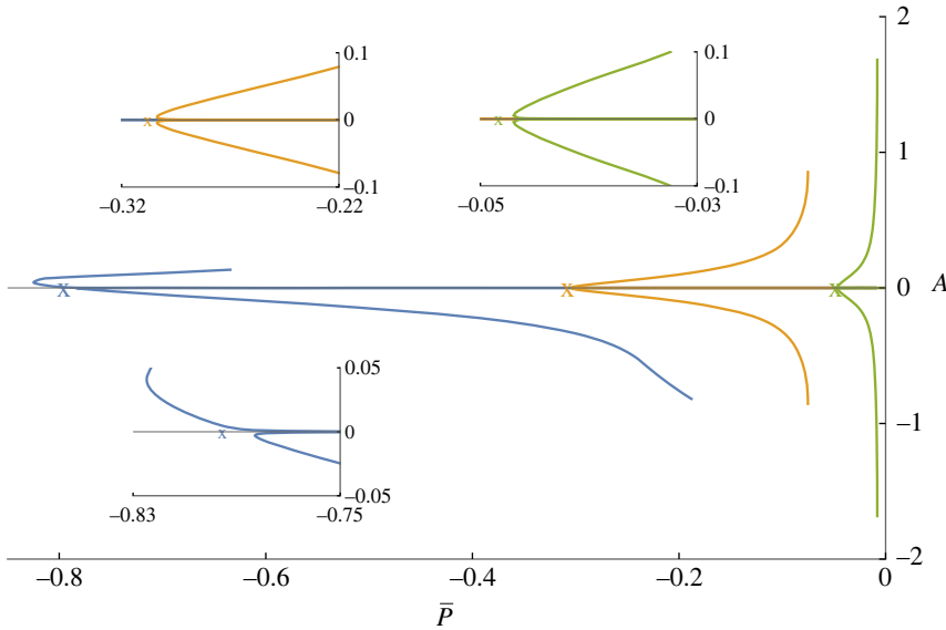
Figure 9. Post-buckling behaviour showing \bar{P} versus the dimensionless amplitude of the deformation at the free surface, setting \bar{V} = 0.3 , \mu^e/\mu^d = 10 , t^d = 0.9 and t^e = 0.9, 0.95, 1 (blue, orange and green lines, respectively). The cross marker denotes the theoretical buckling threshold.
