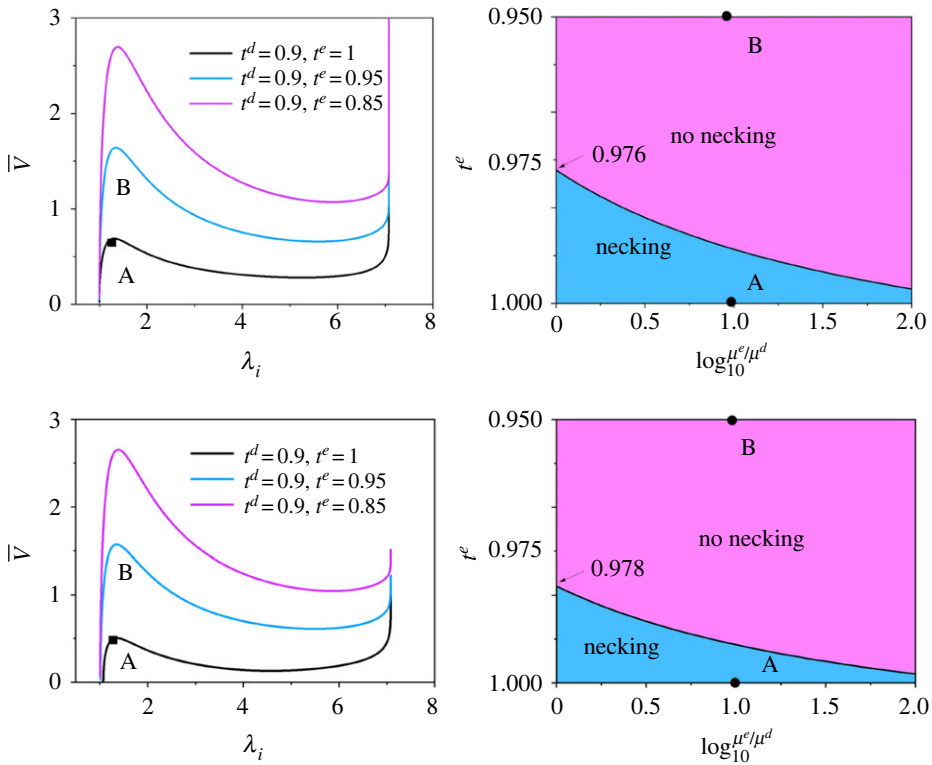
Figure 7. Inflation of voltage-activated ( \bar{P} = 0 top, \bar{P} = 0.06 bottom) dielectric-elastic balloons with t^d = 0.9 and varying t^e . Left: \bar{V} - \lambda_i curve of the balloon at fixed \mu^e / \mu^d = 10 and varying t^e , with the square marker indicating the necking threshold. Right: stability diagram of the balloons with varying t^e and \log_{10} \mu^e / \mu^d . The black, blue and red curves on the left column correspond to three specific balloons: balloon A with t^d = 0.9, t^e = 1 , balloon B with t^d = 0.9, t^e = 0.95 , and balloon C with t^d = 0.9, t^e = 0.85 (balloon C beyond the scope of the phase diagram thus is not presented in the plots on the right).
