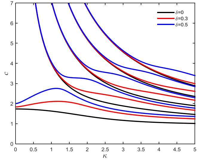
Fig. 3. Phase velocity curves for the first five axisymmetric torsionless wave modes in a solid cylinder.
